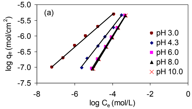
Figure 1: pH effect on 2,4-dinitrophenol adsorption isotherms of NTR 7450 membrane
