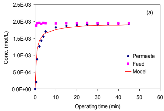
Figure 2: Permeate and feed concentrations of phenol as a function of filtration time for NTR 7450 membrane
