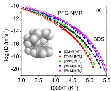
Fig. 1: Diffusion coefficients determined from broadband dielectric spectra by employing the Einstein-Smoluchowski equation (using \omega_c as the characteristic hopping rate) and independently measured by PFG NMR (open symbols). The lines denote fits by the Vogel-Fulcher-Tammann equation. Inset: One of the possible conformations of the [OMIM] cation.
